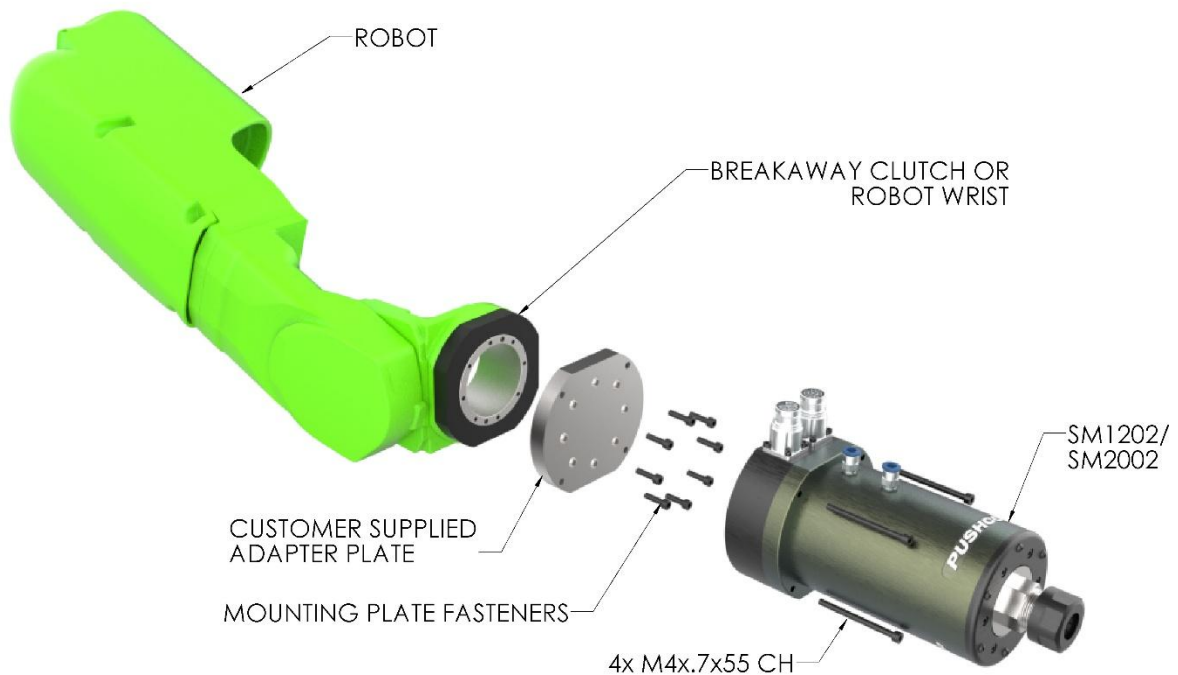
FIGURE 3: RIGID MOUNT
