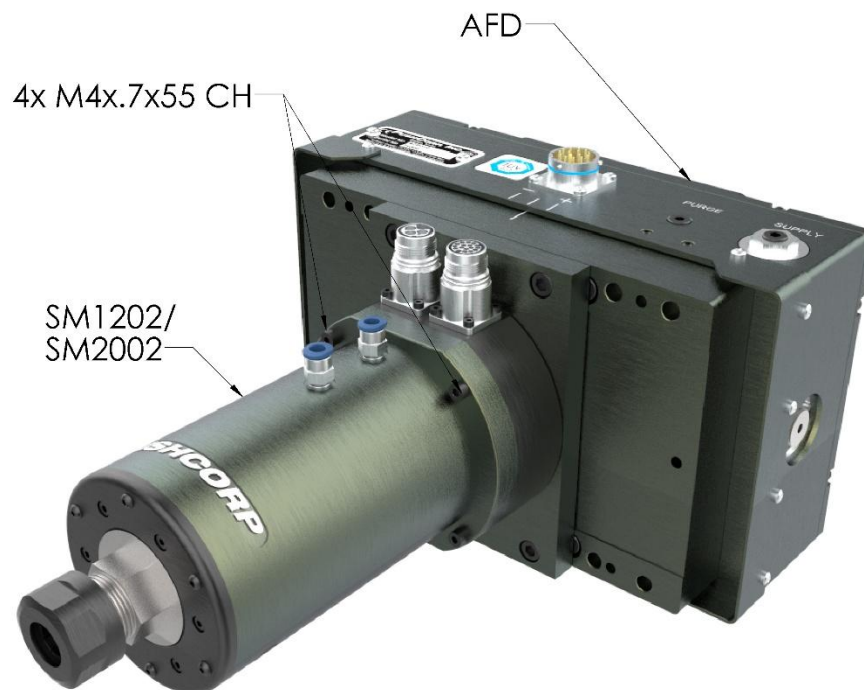
FIGURE 2: PERPENDICULAR MOUNT
