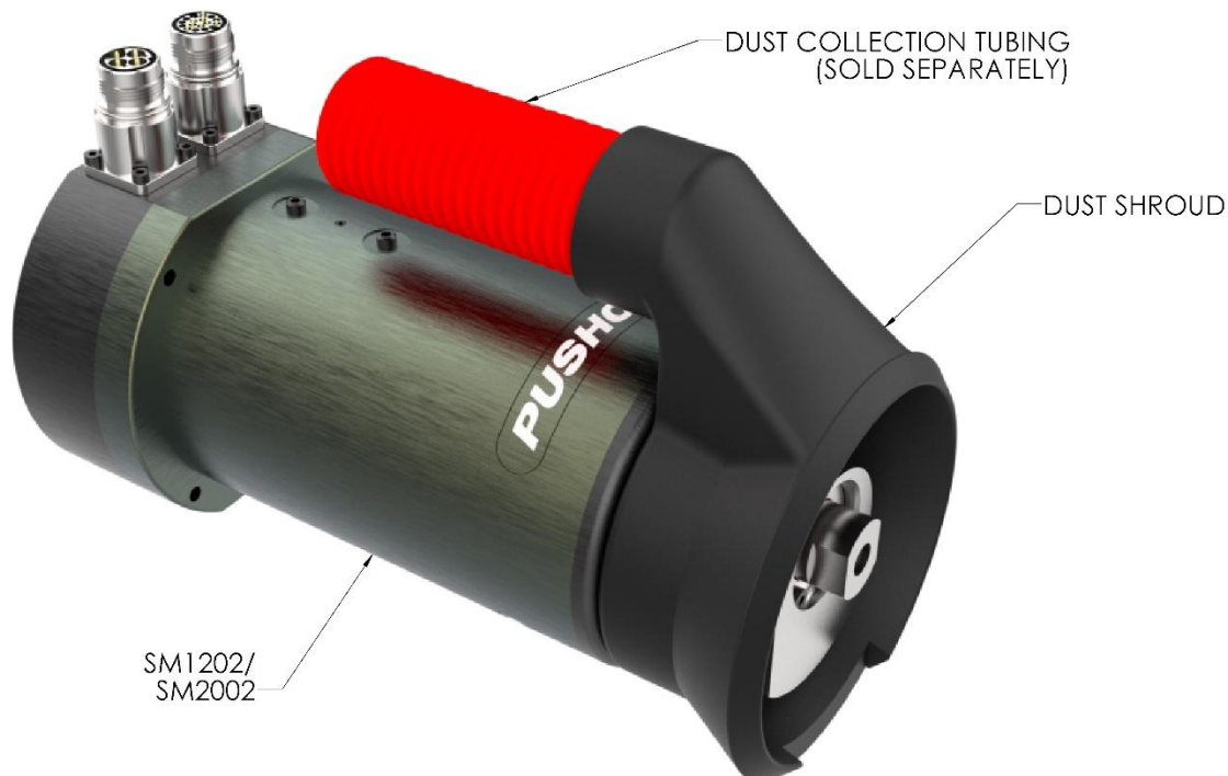
FIGURE 8: DUST COLLECTION SETUP
