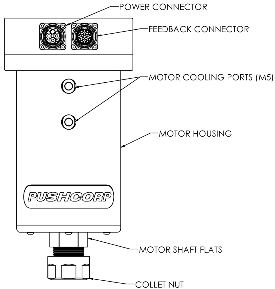
FIGURE 15: SM1202/2002 EXTERNAL FEATURES
