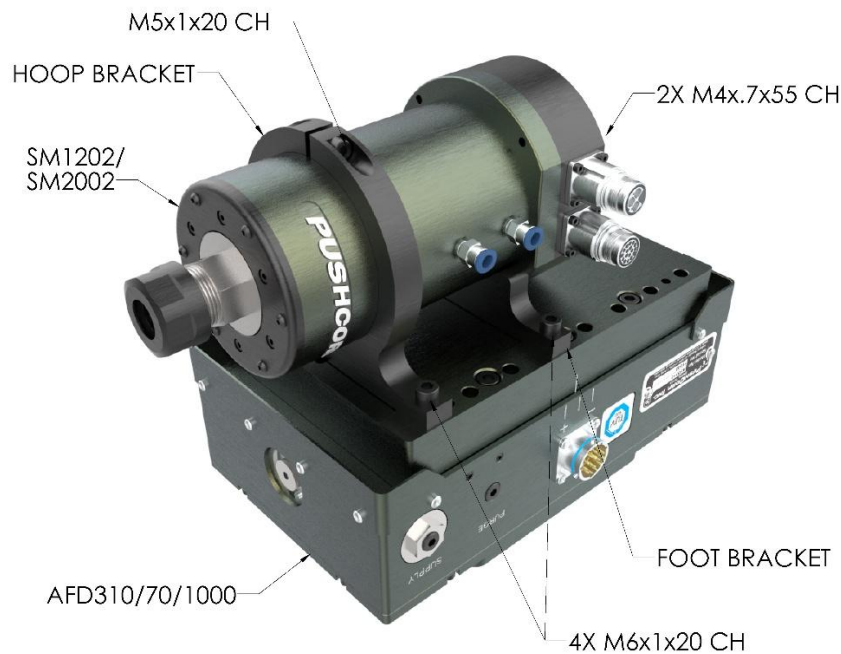
FIGURE 1: PARALLEL MOUNT
